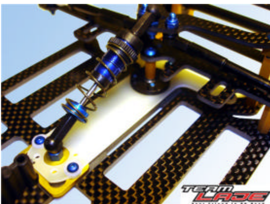
Team Laje's super oil shock and NTS T-bar bracket.
